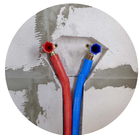
Classic brick process
