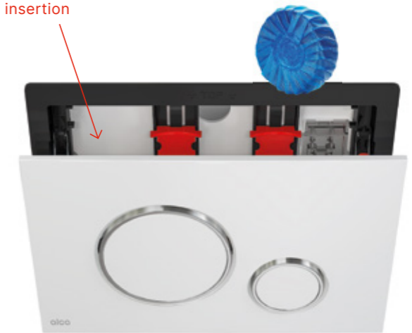
Tilting mechanism of flush plates for easier tablets insertion
